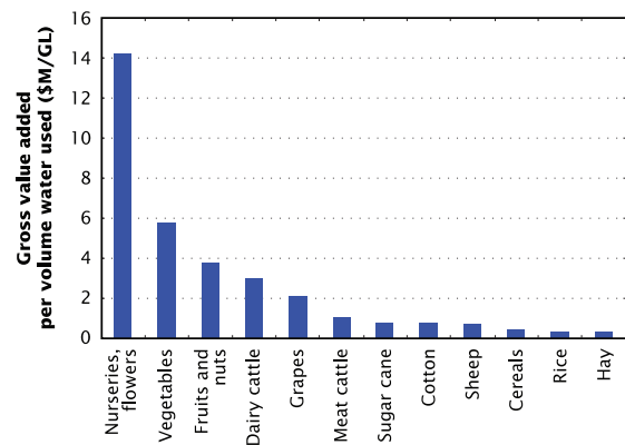
▲ Figure 2.2: Gross value added of irrigated agricultural production across Australia for 2008–09. Nurseries, vegetables, fruits, and nuts produce the highest added value from irrigation. 3
