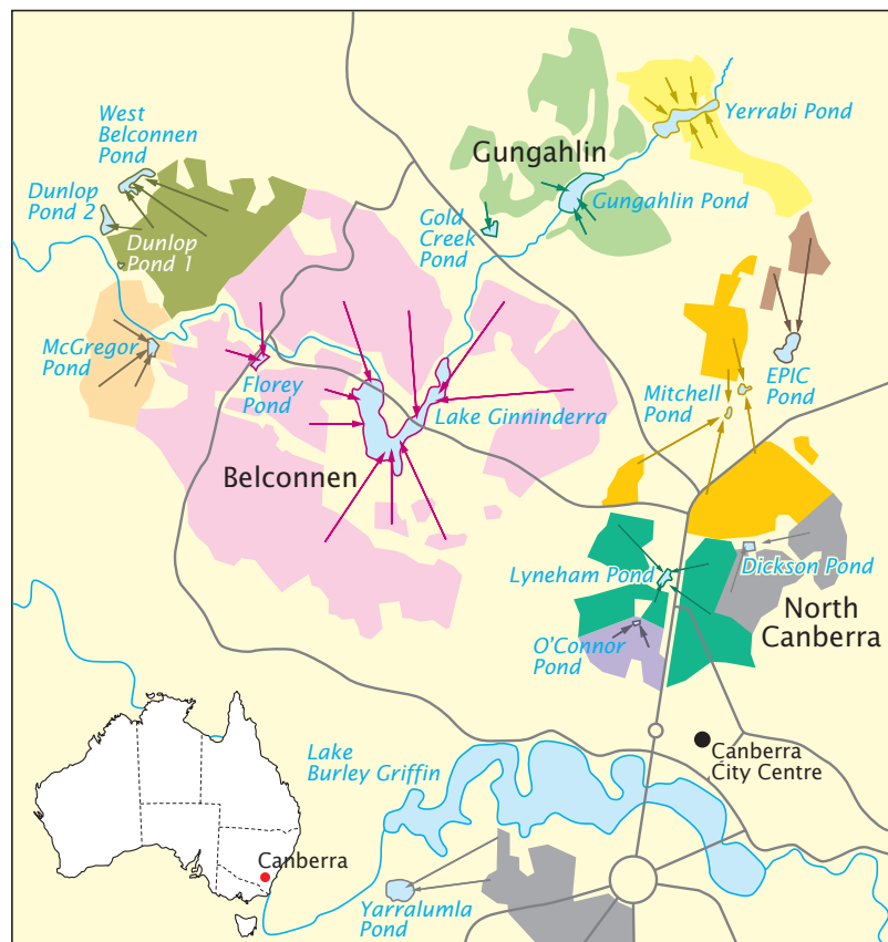
► Figure 7.10: Existing and planned lakes and ponds to capture stormwater in the northern suburbs of Canberra. The storages will be used to provide water for surrounding parks and gardens. 30
