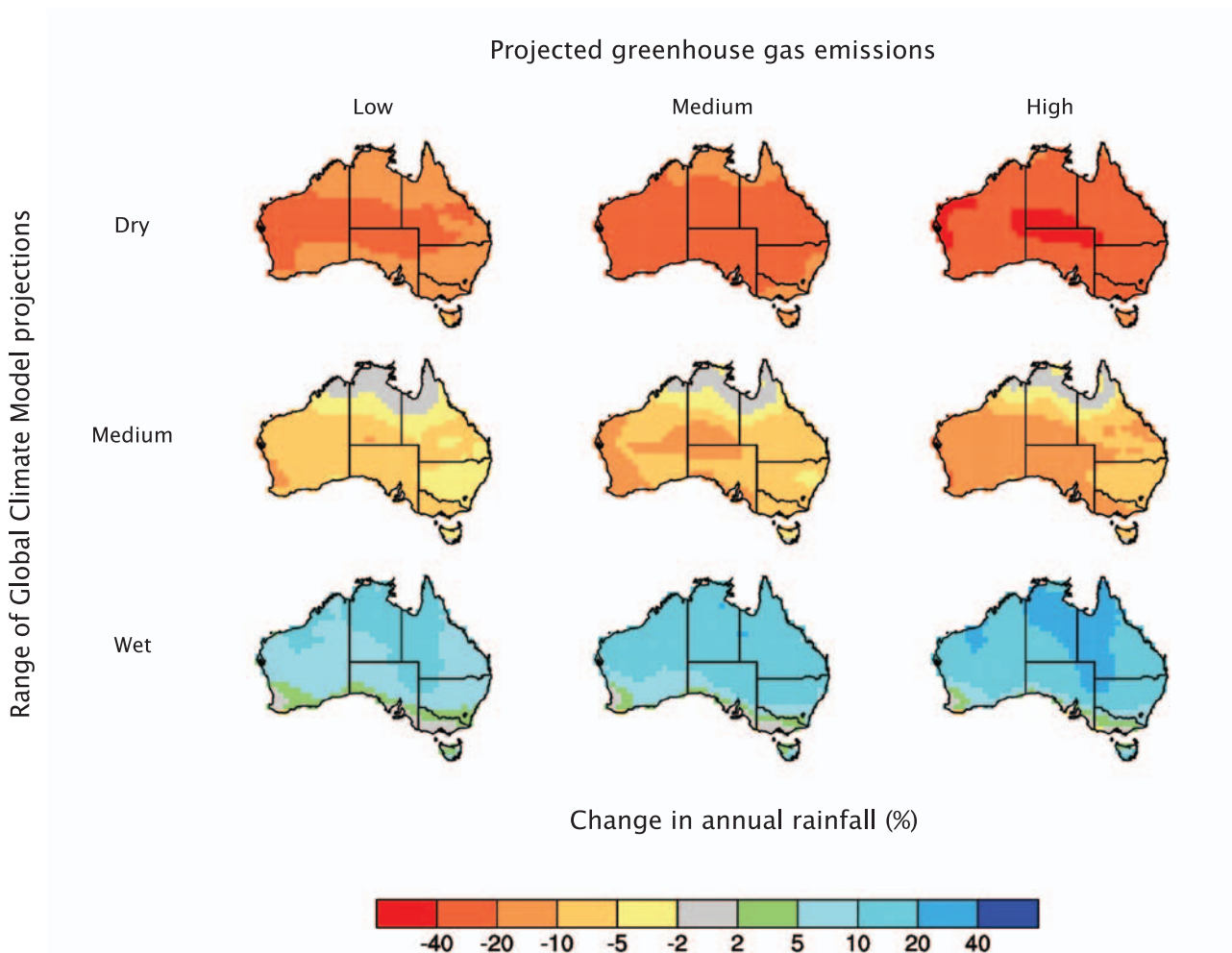
▲ Figure 3.8: Projections for percentage change in average annual rainfall in Australia by 2070 relative to 20th century rainfall. Nine projections are shown. The columns of maps show projections for low, medium, and high future greenhouse gas emissions, showing the effects of different amounts of global warming. The rows of maps show the range of projections from different global climate models. The top row shows the drier model results, the middle row is the mid-range of results and the bottom row shows the wetter projections of average annual rainfall from the models. 26
